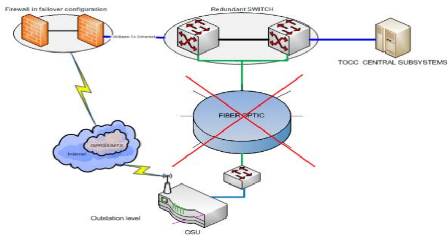
Figure 240: Backup communication network architecture.
